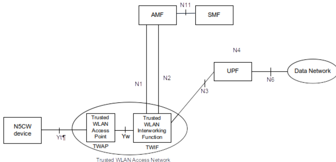
3GPP TS23.501 Figure 4.2.8.5.2-1: Non-roaming and LBO Roaming Architecture for supporting 5GC access from N5CW devices
